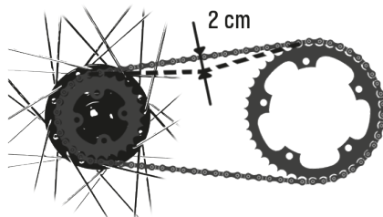
Sl. 4/29 Napetost lanca
