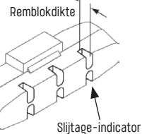
Slijtage-indicator
