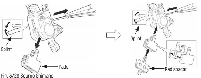
Fig. 3/28 Source Shimano
