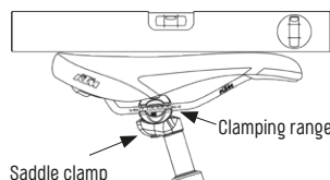
Fig. 4/23 Saddle assembly
