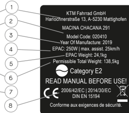
Fig. 2/11 EPAC sticker
