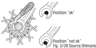
Fig. 3/38 Source Shimano
