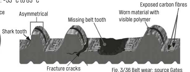
Fig. 3/36 Belt wear; source Gates
