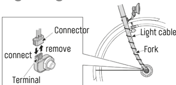
Fig. 2/49 Hub dynamo terminal Source: Shimano
