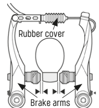
Fig. 3/26 Source Shimano
