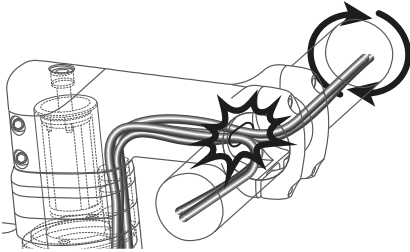
Fig. 1/24 Internally routed brake lines and gear cables
