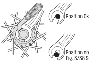
Fig. 3/38 Source Shimano
