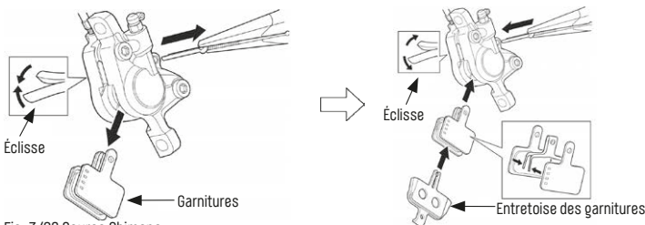
Fig. 3/28 Source Shimano
