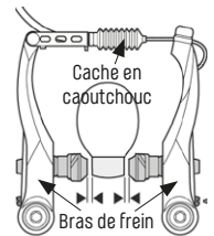
Fig. 3/26 Source Shimano
